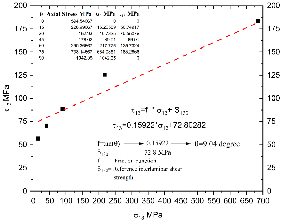
Figure 4.17. Out-of-plane off-axis compression test results
