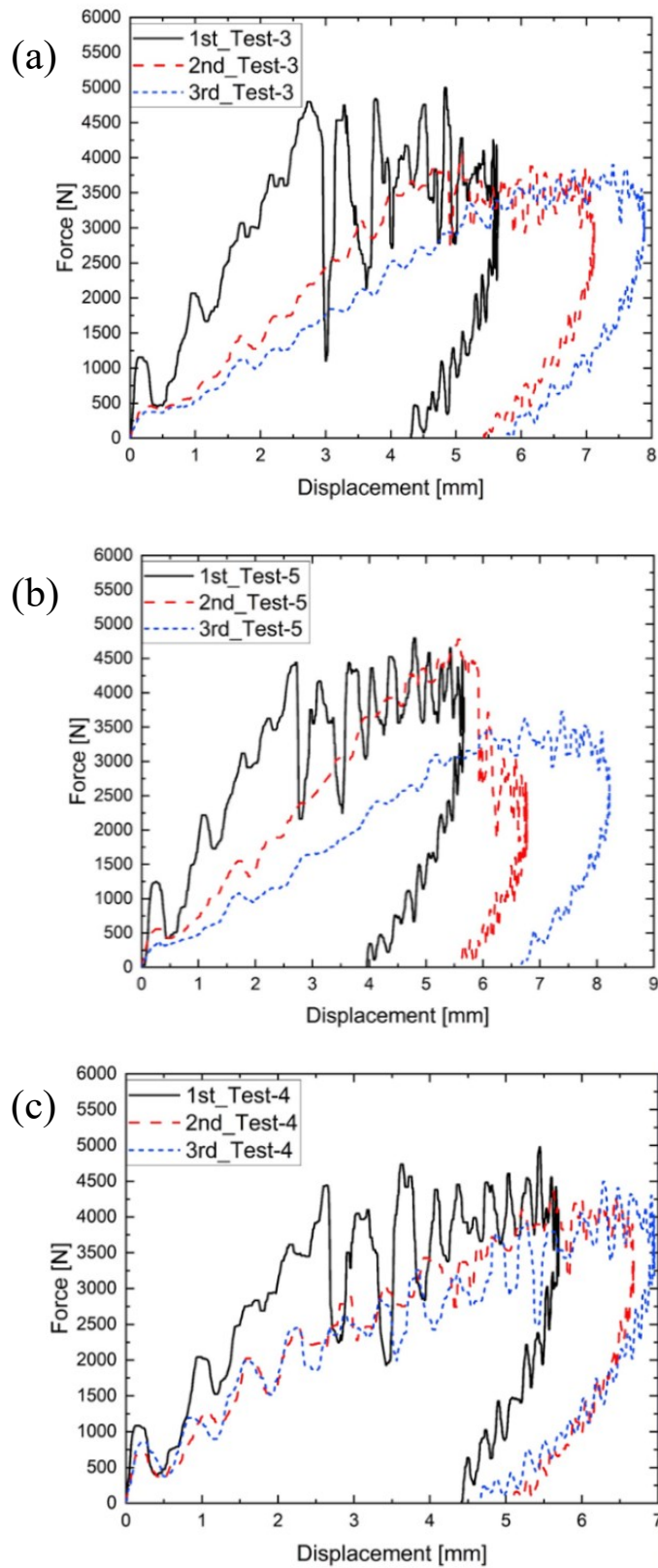
Figure 5.28. Force-displacement curves obtained from the composite subjected to (a),(b) multiple impacts at the same location and (c) impacts at the different locations
