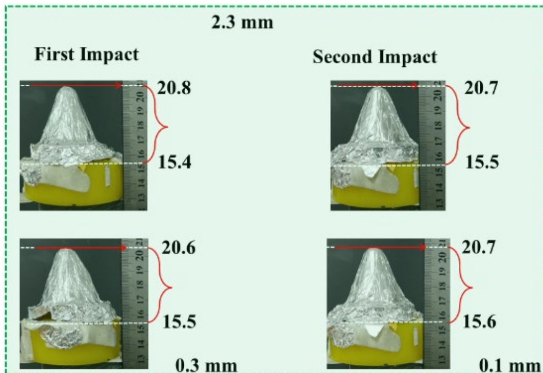
Figure 4.21. The back surface displacement measurement of the carbon composite with a thickness of 2.3 mm
