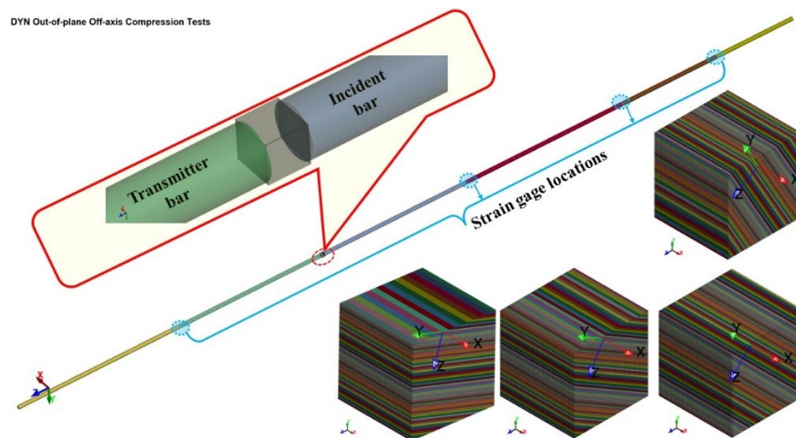
Figure 3.13. Simulation of dynamic compression tests of out-of-plane off-axis samples
