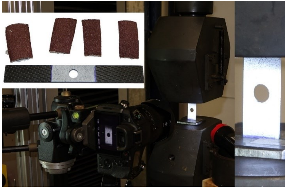
Figure 2.25. Open-Hole Tensile Tests
