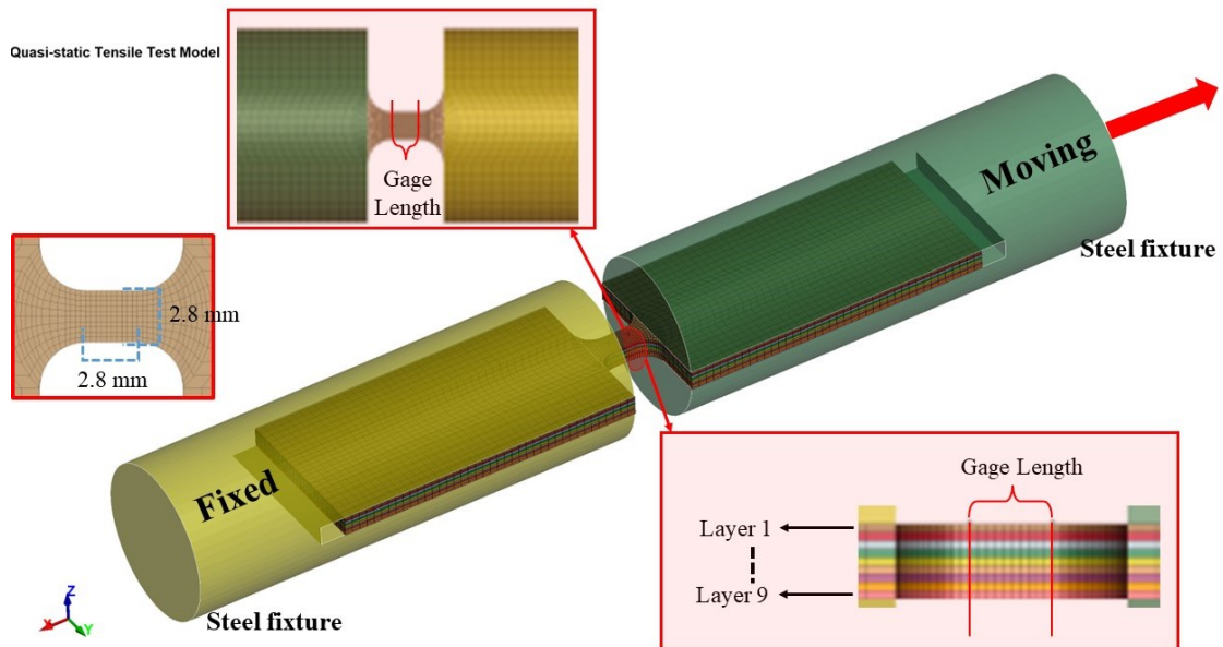
Figure 3.6. Quasi-static tensile test model
