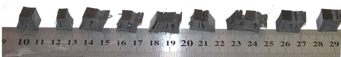
Figure B.3. (a) The deformation results of cubic samples in the weft direction over time at different strain rates and (b) the failed cubic samples in the weft direction
