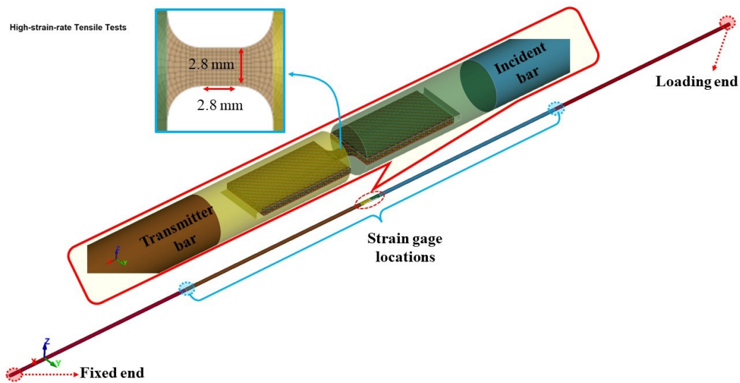
Figure 3.7. High-strain rate tensile test model
