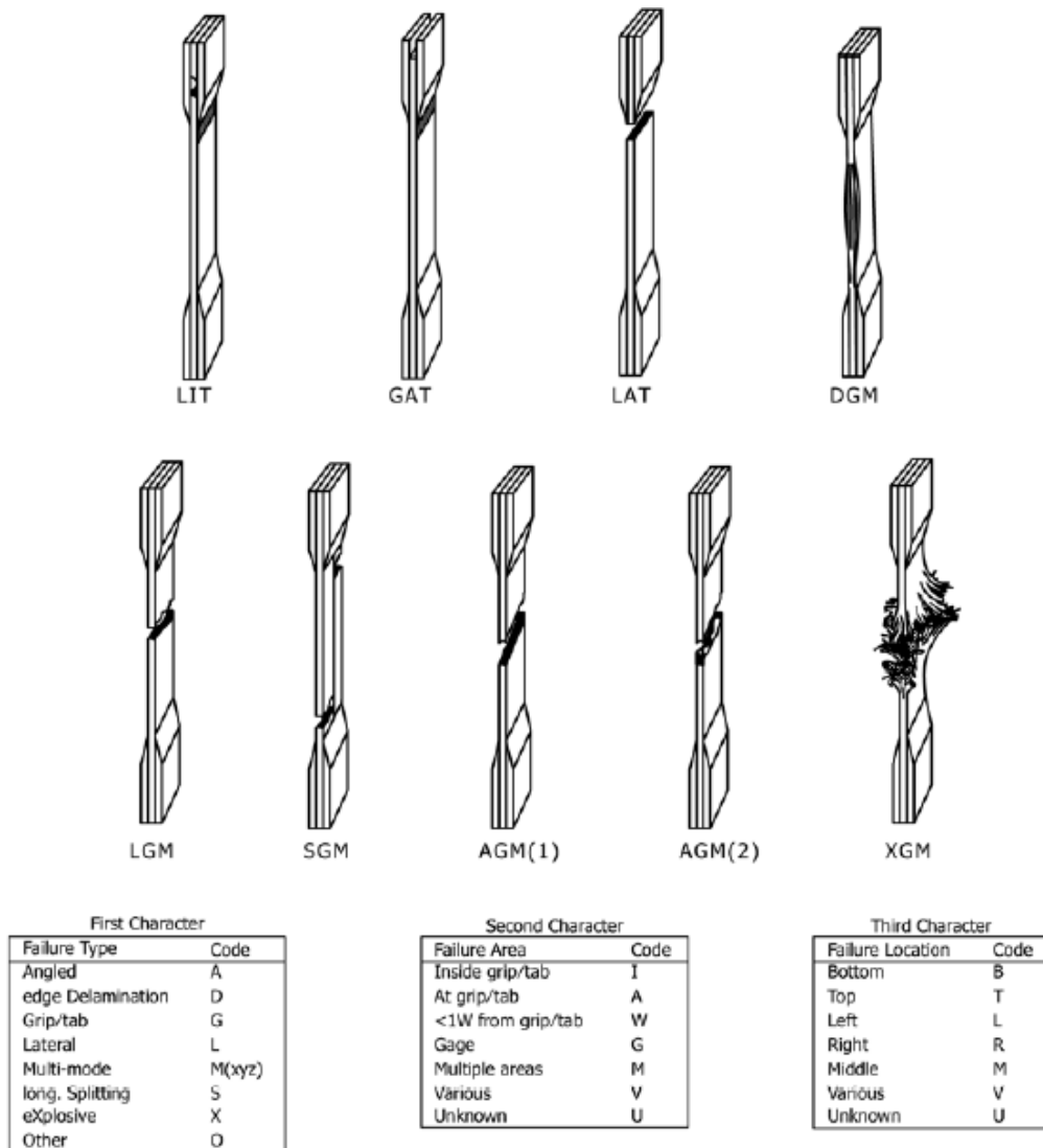
Figure A.1. Tensile specimen failure identification (Source: ASTM D3039 2 )
