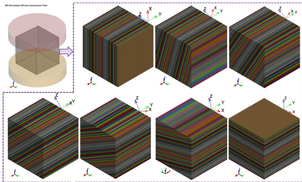
Figure 3.12. Numerical quasi-static compression tests of out-of-plane off-axis samples
