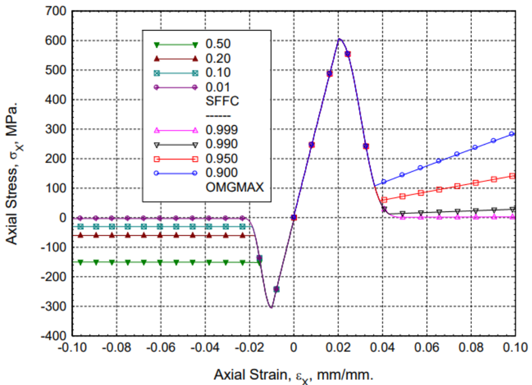
Figure 3.2. The effect of OMGMX and SFFC parameters on a stress-strain curve
