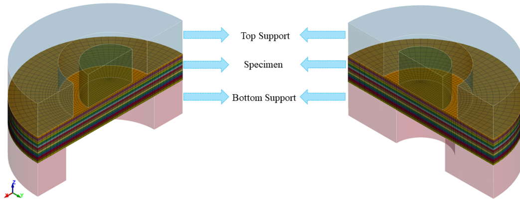
Figure 3.14. Quasi-static punch shear test models
