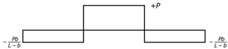
Force Diagram
