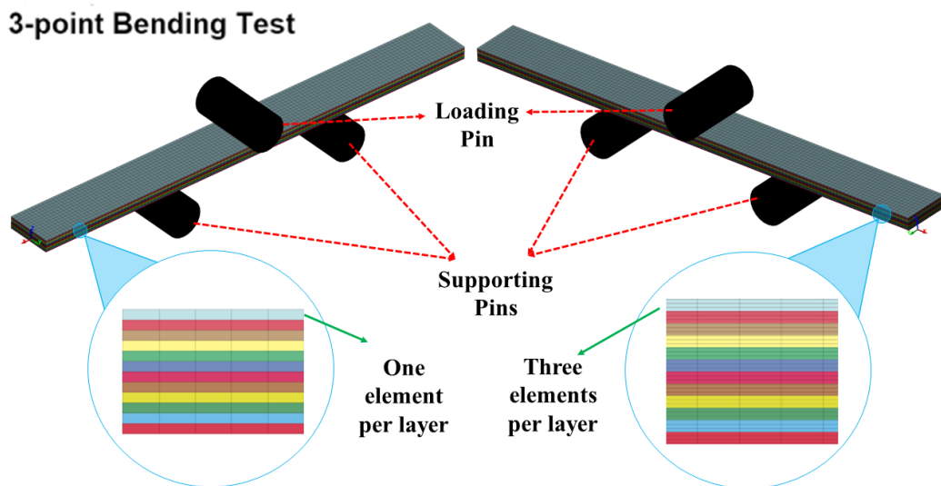
Figure 3.15. 3-point bending test models using solid elements
