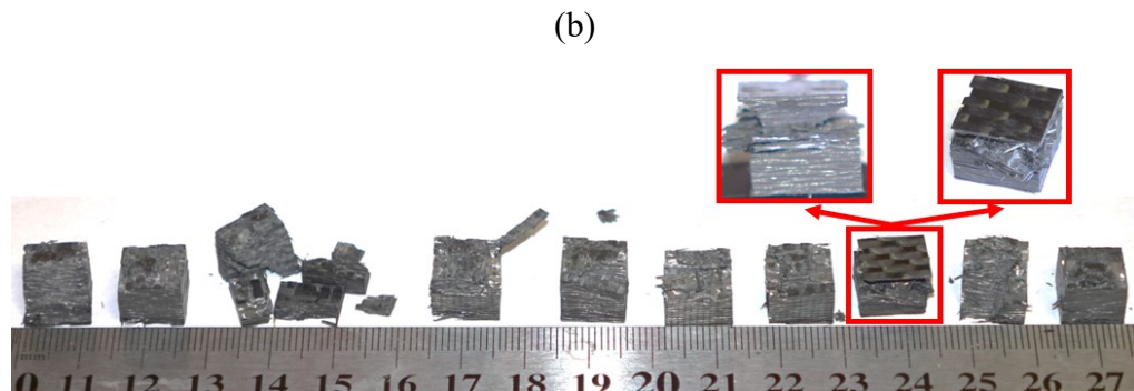
Figure B.4. (a) The deformation results of cubic samples in the warp direction over time at different strain rates, the failed cubic samples (b) in the warp and (c) in the thickness direction
