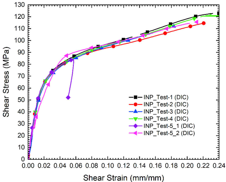
Figure 4.11. In-plane shear results
