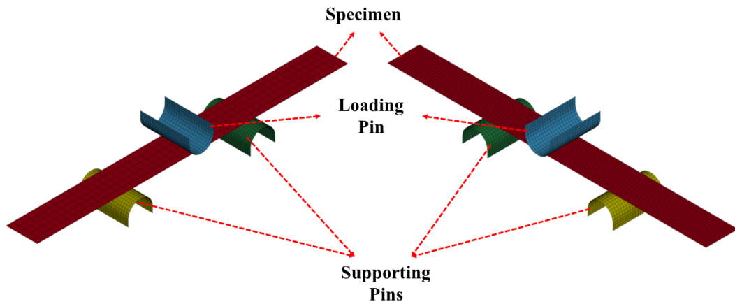
Figure 3.16. 3-point bending test models using shell elements
