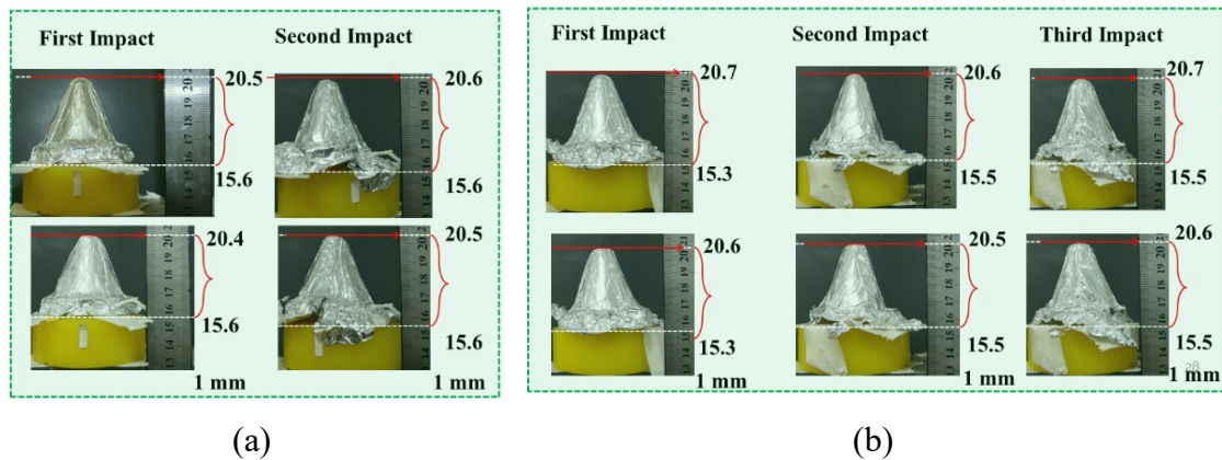
Figure 4.20. The back surface displacement measurement of the carbon composite with a thickness of 0.88 mm (a) Test-1 and (b) Test-2
