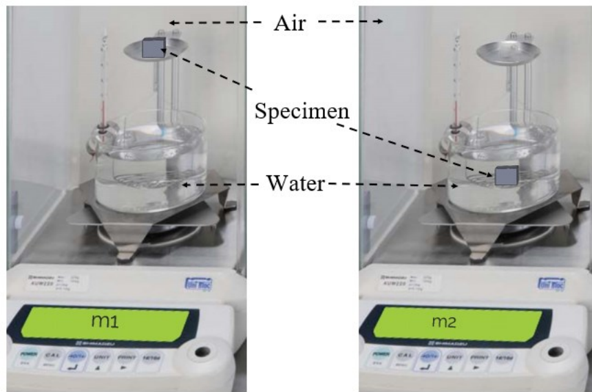
Figure 2.5. Density measurement system
