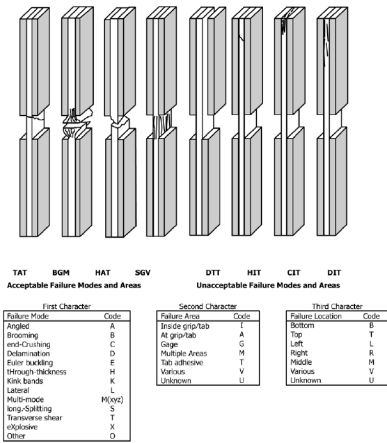
Figure A.2. Compression specimen failure identification (Source: ASTM D6641 56 )
