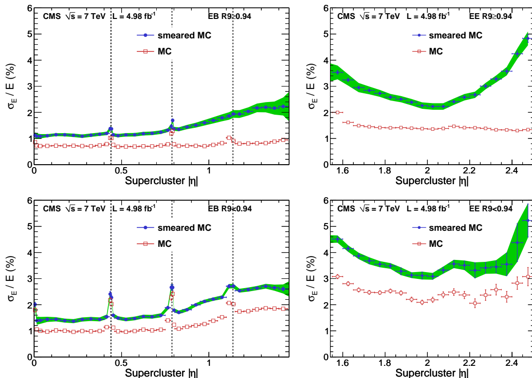
Figure 15. Photon energy resolution in bins of pseudorapidity |\eta| for the barrel (left column) and the endcaps (right column). The resolution is shown separately for photons having R_9 \geq 0.94 (top row) and R_9 < 0.94 (bottom row). The energy resolution is plotted for the simulated H \rightarrow \gamma\gamma events for the default MC simulation and for MC simulation with the addition of Gaussian smearing. The green band shows the uncertainty on the photon resolution calculated as the quadratic sum of the uncertainty on the smearing term and the statistical uncertainty in the photon resolution (shown by the vertical error bars).
