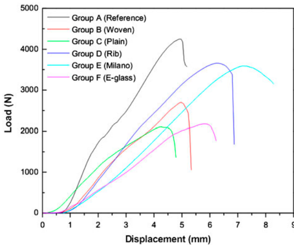
Figure 4. Load-displacement curves of PCP wrapped in various configurations.
