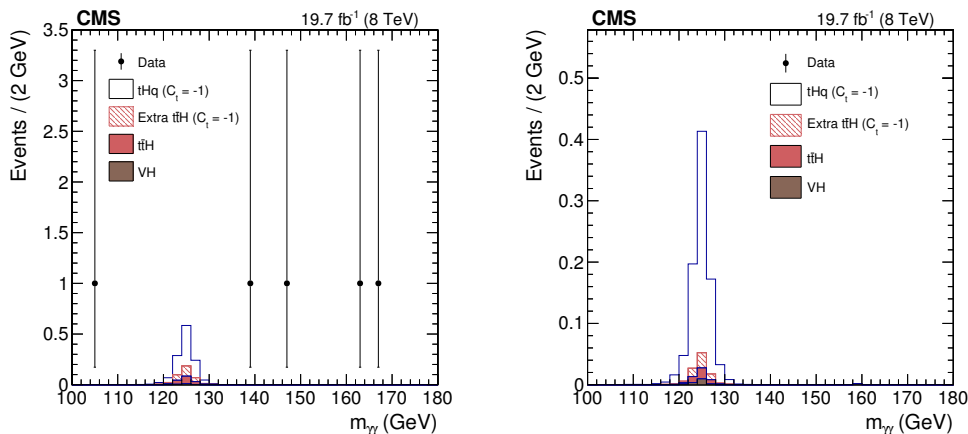
Figure 2. Invariant mass of the diphoton system for events passing the event selection requirements, but for the likelihood discriminant cut (left), and for events passing the full selection (right). The data (black markers) are compared to the MC simulation (stacked histograms). No events are observed after the requirement on the likelihood discriminant.
