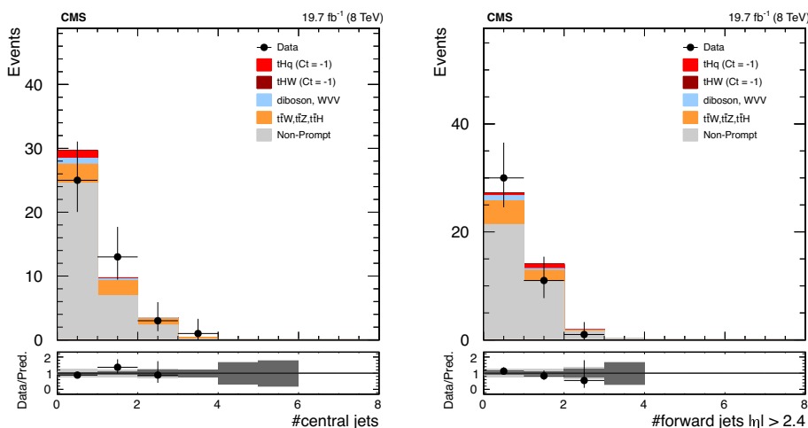
Figure 10. Sample of input variables to the final discriminant in the H \rightarrow WW analysis. Left: distribution of the number of central jets. Right: distribution of the number of forward jets. The signal contribution is normalized to the prediction of the anomalous coupling hypothesis and stacked on top of the predicted background contributions. The bottom panels show the ratio between data and predictions, together with the statistical and systematic uncertainty bands.
