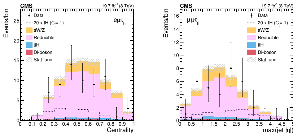
Figure 11. Sample of input variables to the final discriminant in the H \rightarrow \tau\tau analysis. The distributions are shown for events failing the tight electron and muon isolation criteria. Left: distribution of the centrality for events with an electron, a muon, and a hadronically-decaying tau lepton. Right: distribution of the rapidity of the most forward jet in events with two muons and a hadronically-decaying tau lepton. The dashed line shows the expected contribution from the tHq signal ( C_t = -1 ) case, multiplied by 20.
