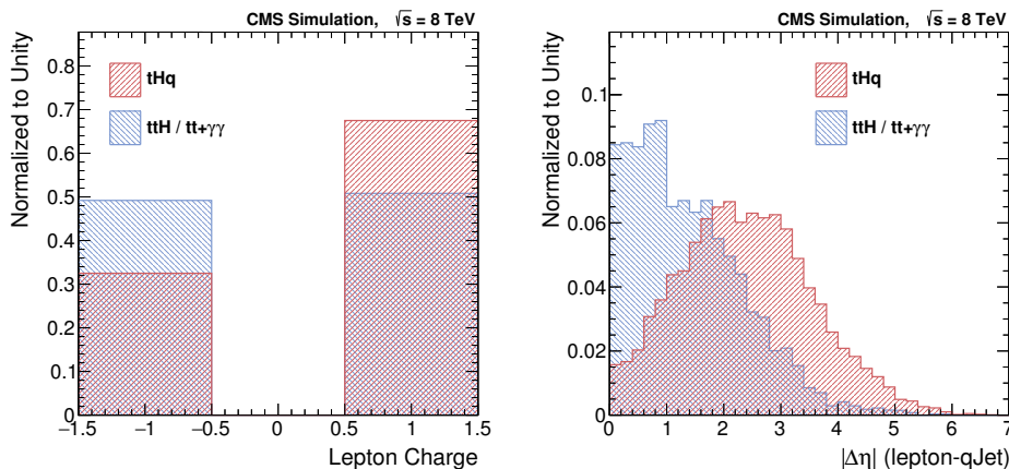
Figure 8. Sample of input variables to the final discriminant in the H \rightarrow \gamma\gamma analysis. Left: distribution of the electric charge of the reconstructed lepton. Right: distribution of the pseudorapidity difference between the lepton and the forward jet. Both plots are shown after the initial kinematic selection, and both distributions are normalized to unit area.
