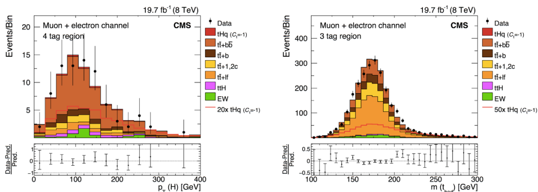
Figure 9. Sample of input variables to the final discriminant in the H \rightarrow b\bar{b} channel. Left: distribution of the reconstructed transverse momentum of the b\bar{b} system in the signal hypothesis for events with an high transverse momentum electron or muon and four b-tagged jets. Right: distribution of the invariant mass of the tri-jet system under the hypothesis of the presence of a hadronically-decaying top quark for electron/muon events with exactly three b-tagged jets. In both cases the signal is normalized to the rate for the analogous coupling hypothesis, and is shown stacked on top of the SM background prediction. It is also shown as a separate histogram, magnified by a factor of 20 (50) in the four-tag (three-tag) sample to enhance visibility.
