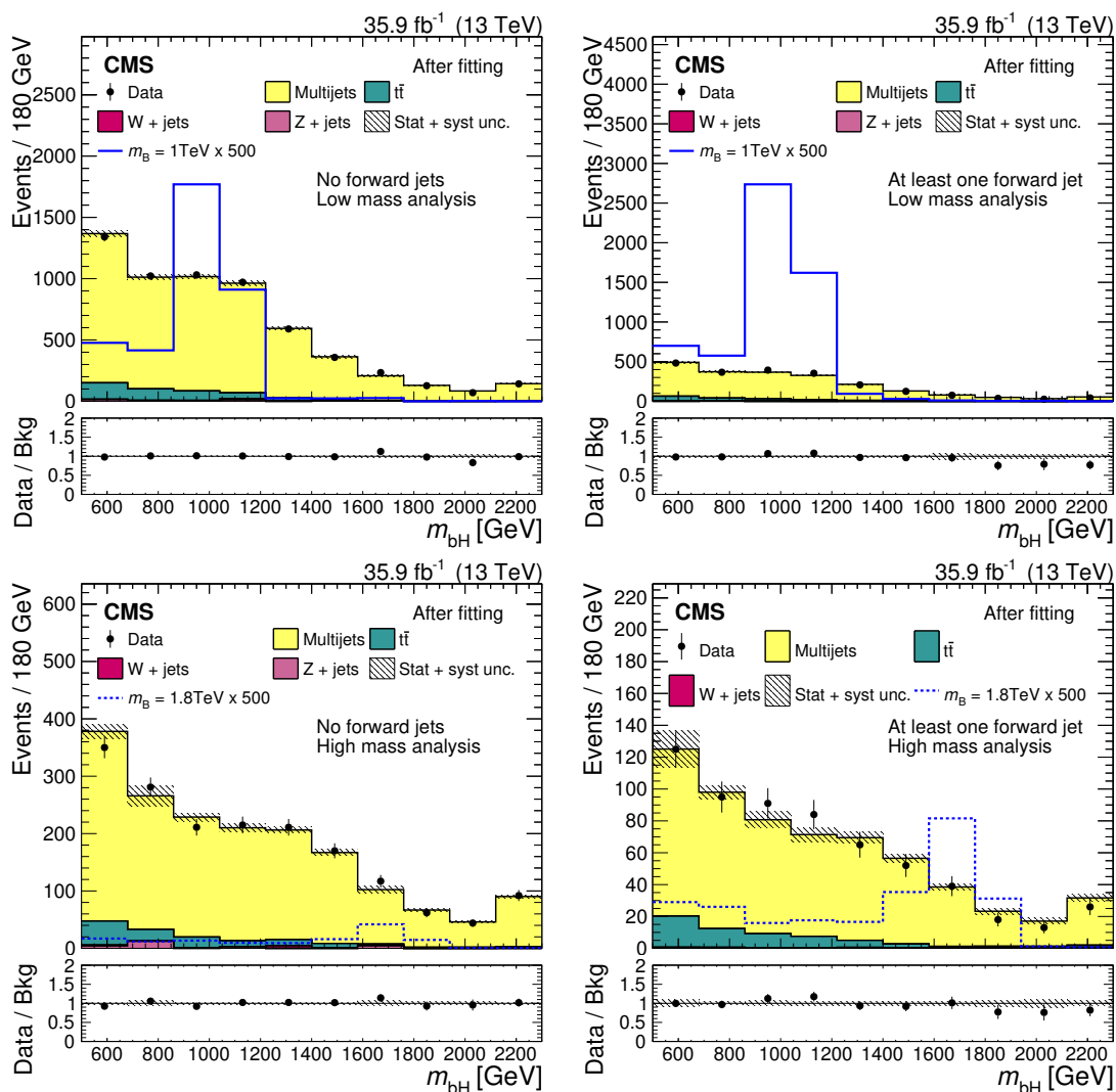
Figure 5. Distribution in the reconstructed B quark mass after applying all selections to events with no forward jets (left) and to events with at least one forward jet (right), compared to the background distributions estimated after fitting. The upper and lower plots refer to the low- and high- m_B analyses, respectively. The expectations for signal MC events are given by the blue lines. The different background contributions are indicated by the colour-filled histograms, and are obtained from Monte Carlo simulation, except for the multijets component, which is derived from data. The grey-hatched error band shows total uncertainties in the background expectation. The ratios of the observations to background expectations are given in the lower panels, together with the total uncertainties after fitting, indicated by the grey-hatched band.
