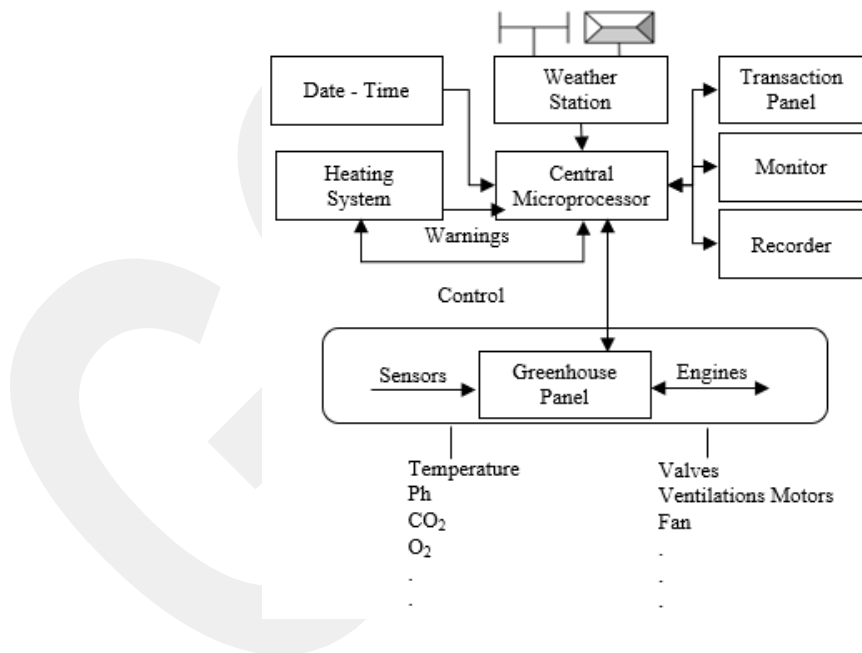
Figure 3.7. Automation Schema for Sample Greenhouse Design
